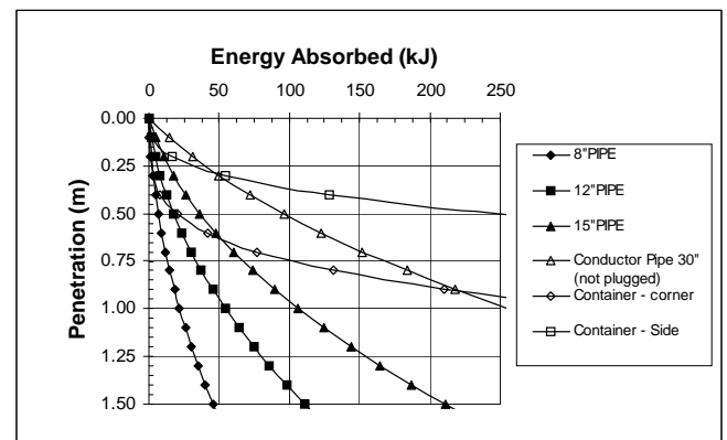
Figure 6 Absorbed energy in gravel
