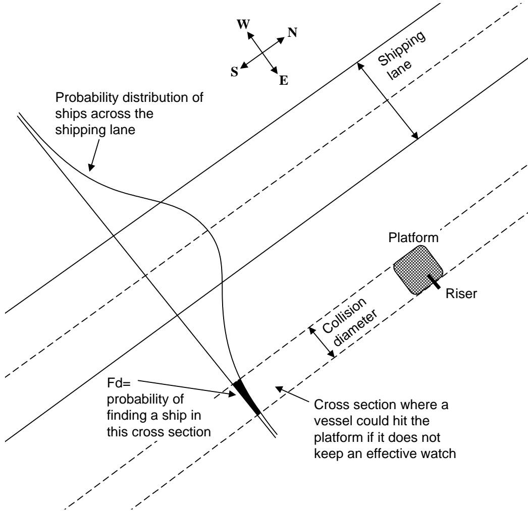
Figure 11 Normal distributed geometric collision probability
