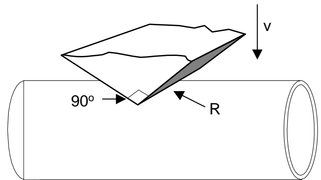
Figure B1 Profile for deciding impact capacity.
