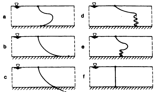
Figure 7 Observed fall-patterns for dropped pipe joints in water (Aanesland, 1987)
