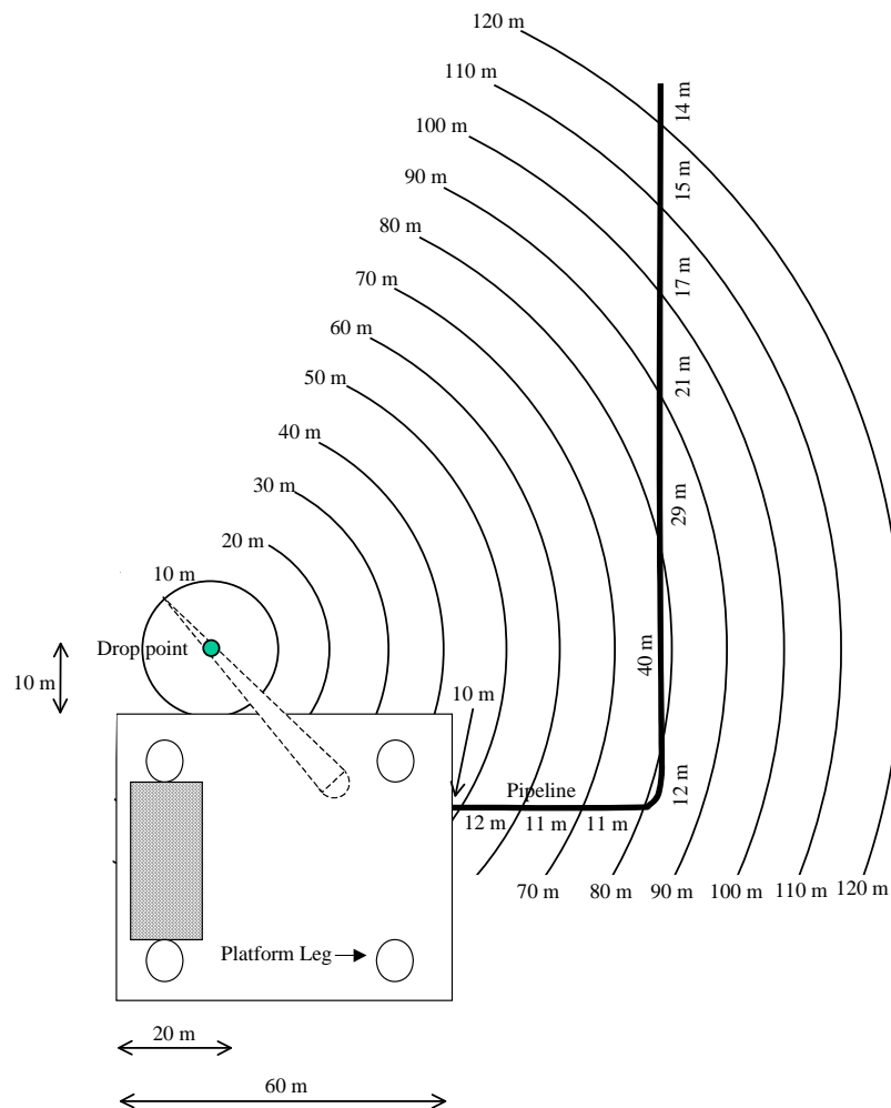
Figure A2 Field Layout with indication of 10-metre interval rings for calculating the object excursion and hit probability.
