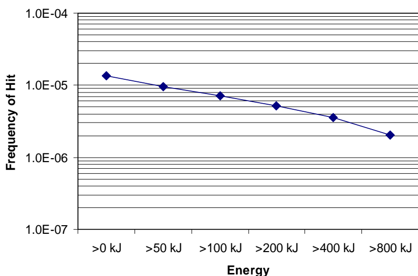
Figure A3 Accumulated annual hit frequency for different impact energy levels.
