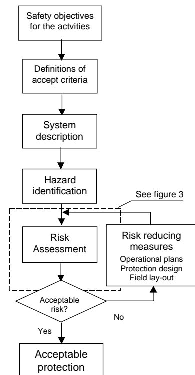
Figure 2 Process Description of the Pipeline Protection Assessment.
