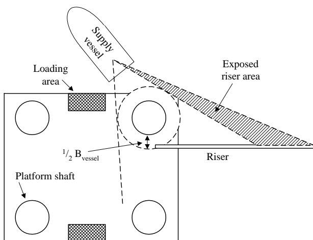
Figure 12 Catenary riser area exposed to supply vessel collision during loading/unloading.
