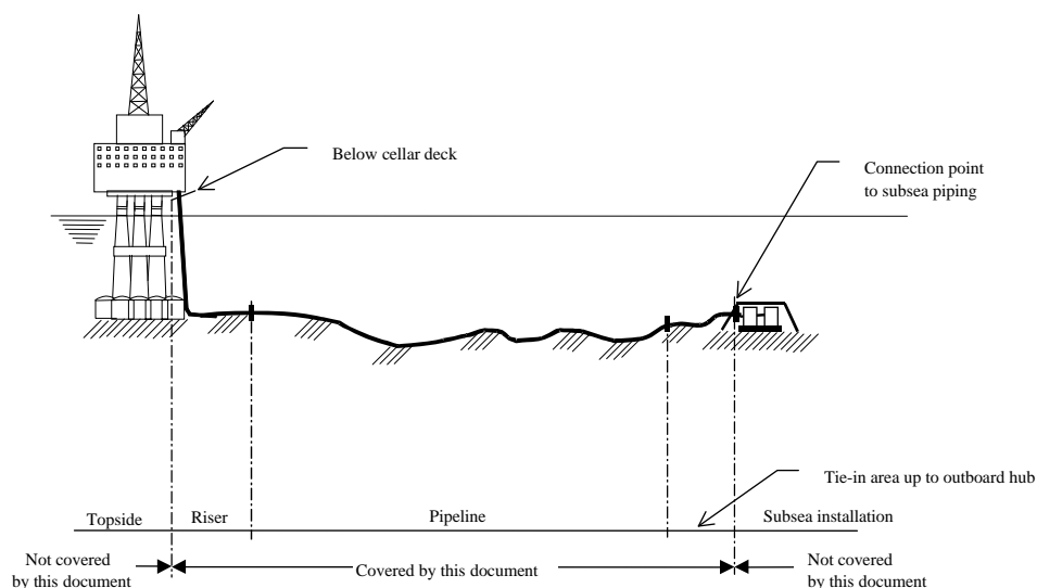
Figure 1 Application of the recommended practice
