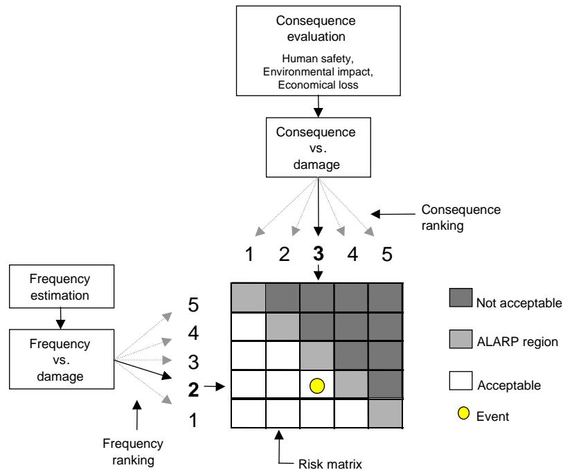
Figure 3 Process description of a risk assessment (Figure is only schematic, actual acceptable limits need to be given by operator)
