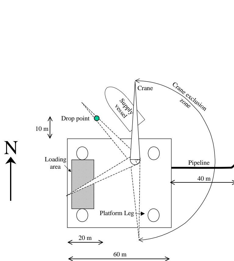
Figure A1 Field layout.
