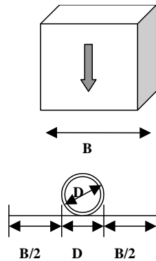
Figure 10 Definition of Hit Area
