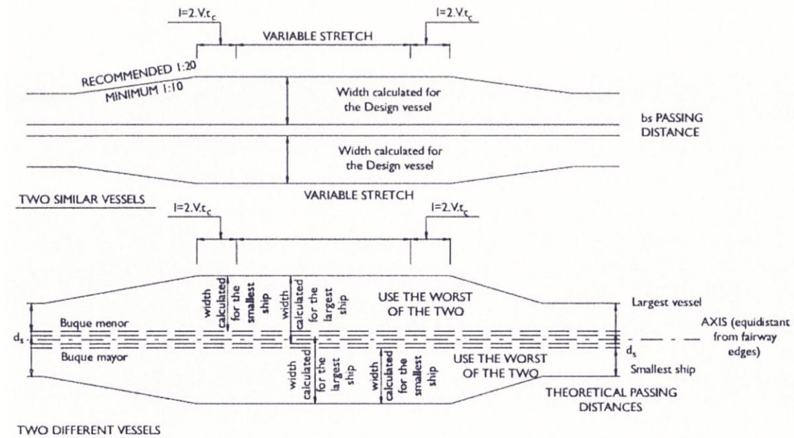
Figure G1-9: Configuration, straight stretches with varying environmental conditions, two lanes
