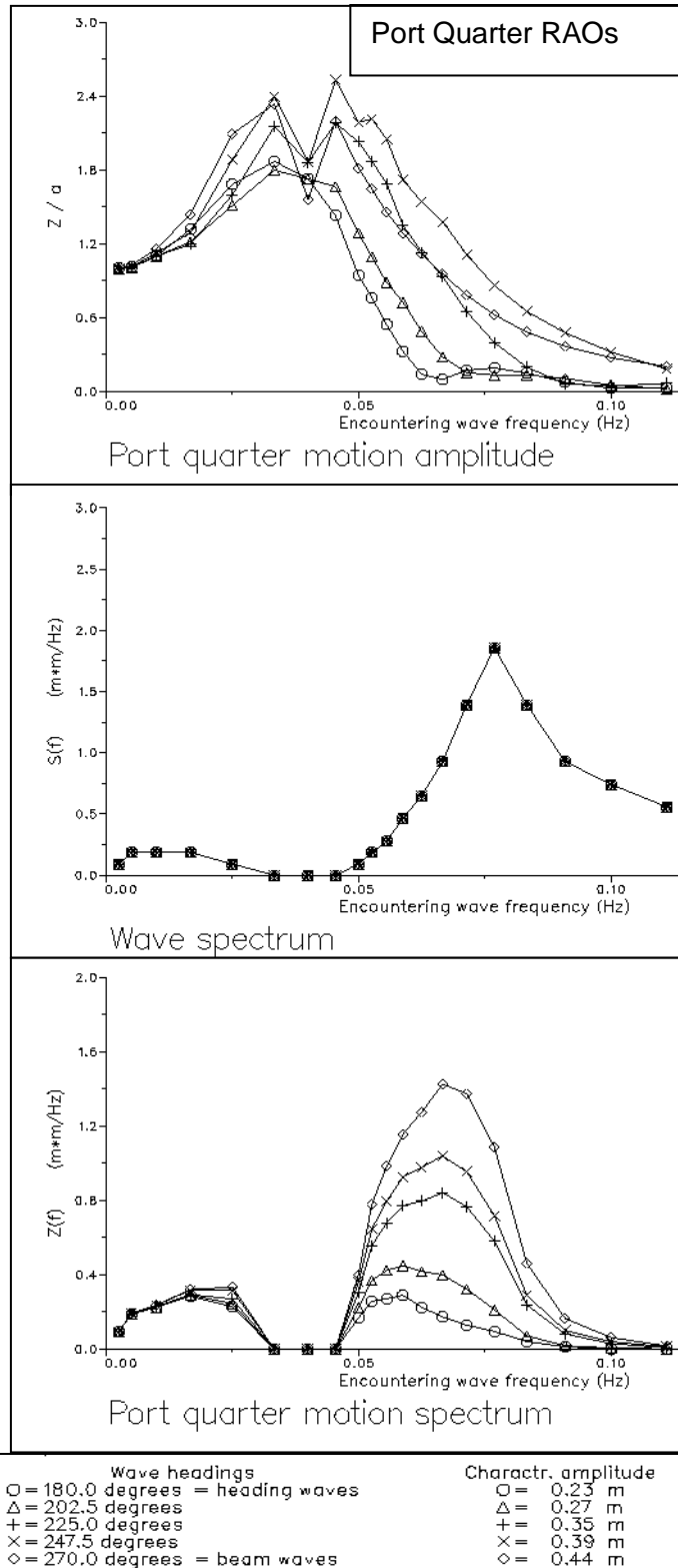
Figure 2.11: Port quartering RAO, wave spectrum, motion spectrum and significant (characteristic) vertical motion amplitude for heave, roll and pitch motions. This example is for Hm_0 = 1 m
