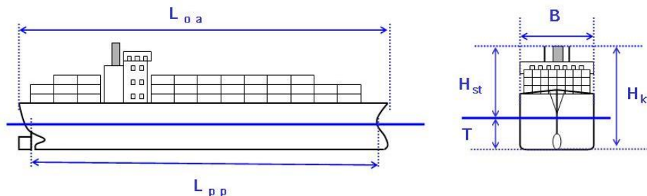
Figure 1.2: Typical ship dimensions
