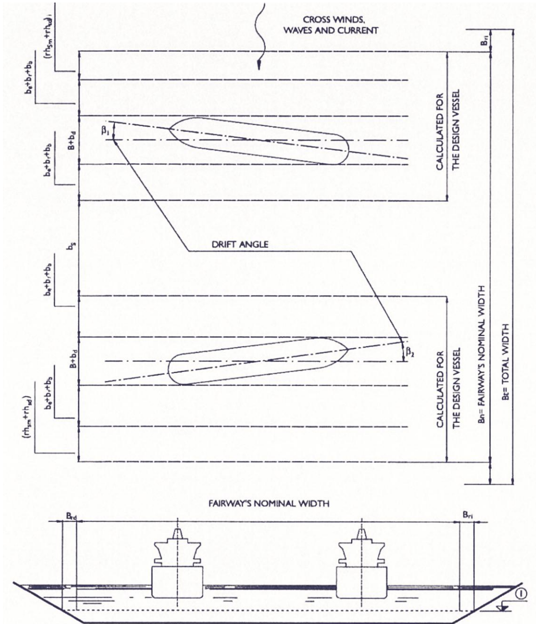
Figure G1-7: Width for straight stretch fairways with two navigation lanes. Operation with the same tonnage.
