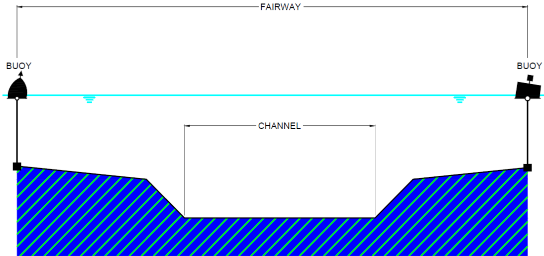
Figure 3.1: Channel and fairway definition (where channel is defined by the channel bed width or width at nominal bed level)
