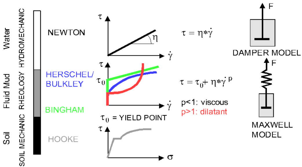
Figure E-1: Rheological properties of mud [Kerckaert et al., 1985 ; Wurpts & Torn, 2005]
