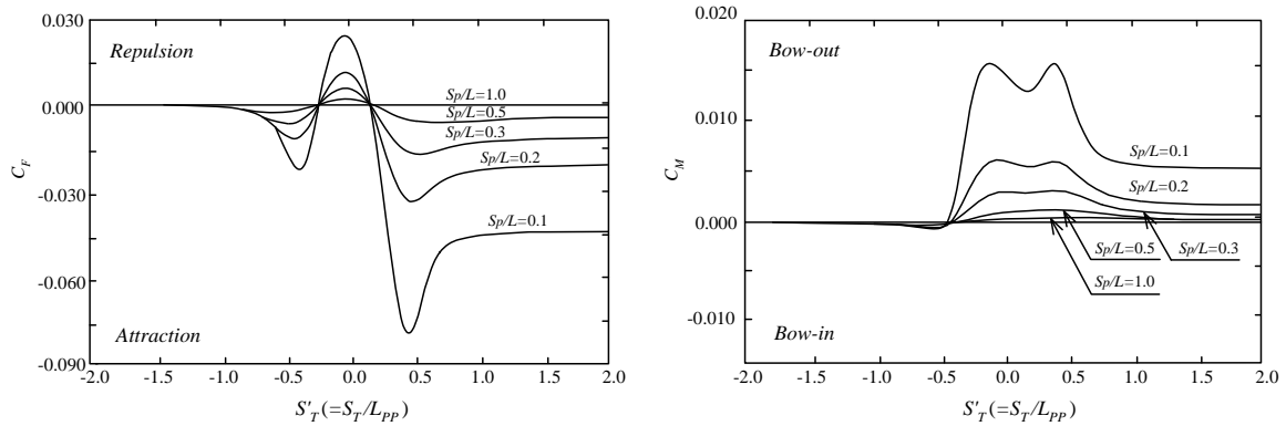
Figure G2-2: Lateral force and yaw moment due to bank effects
