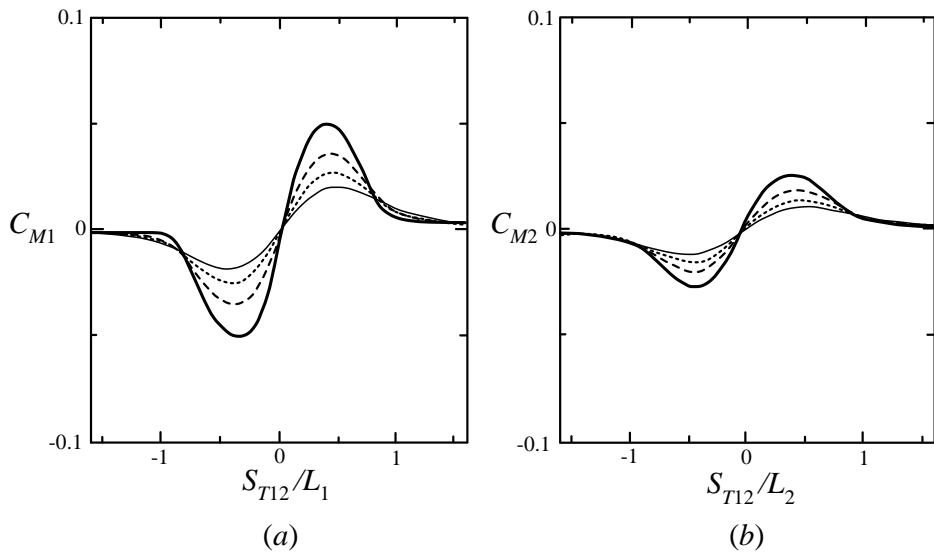
Figure G2-4: Yaw moment due to two-ship interaction in overtaking
