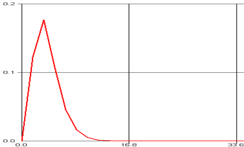
Figure 3.21: Erlang-k with \mu = 4, k = 4
