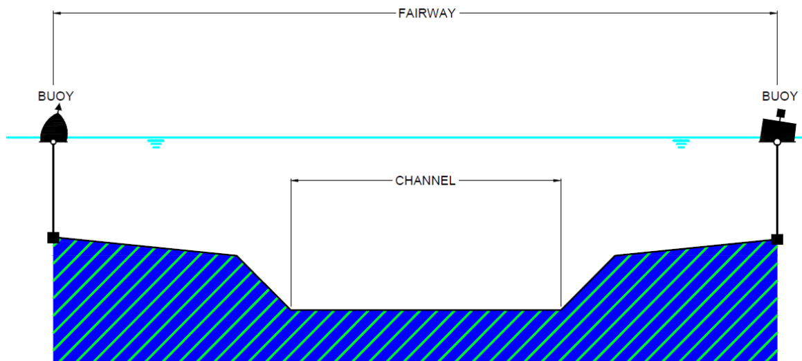
Figure 1.1: Channel and fairway definition
