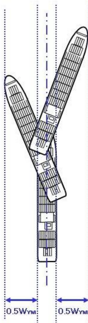
Figure G2-2: W_{YM} : Width requisite against yawing motion
