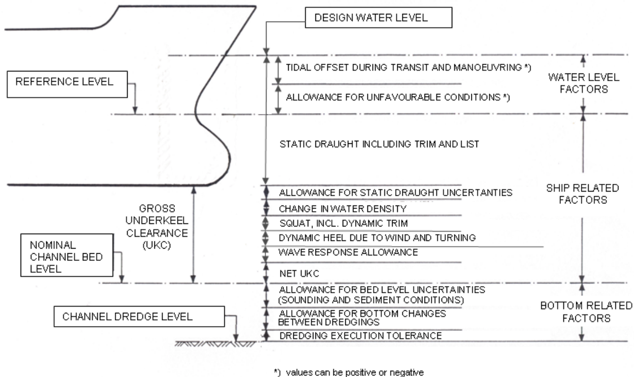
Figure 2.1: Channel depth factors
