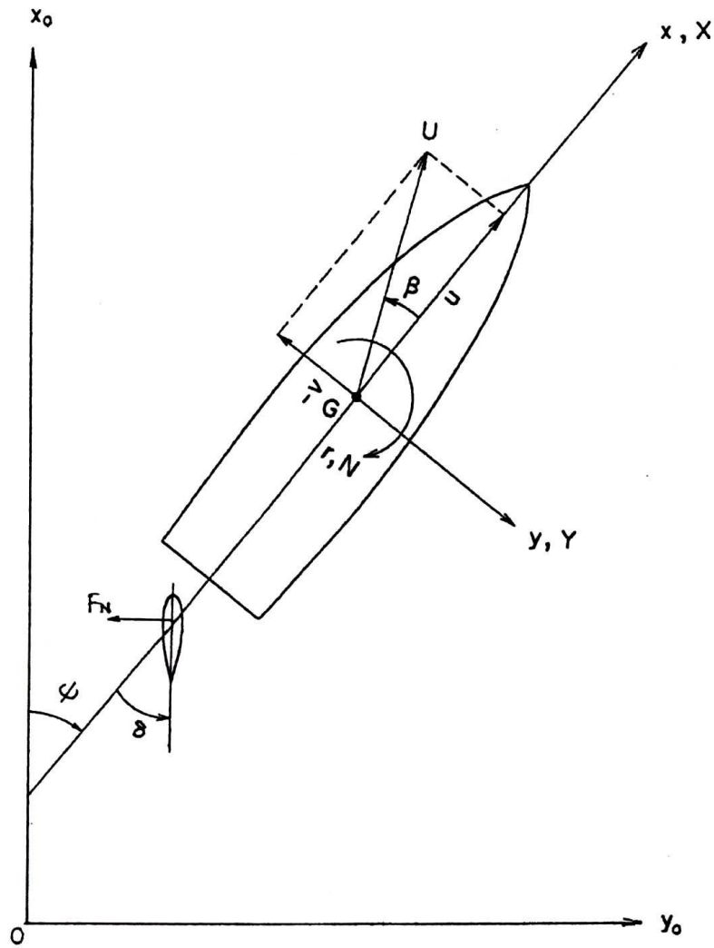
Figure G3-1: Coordinate system of ship manoeuvring motion
