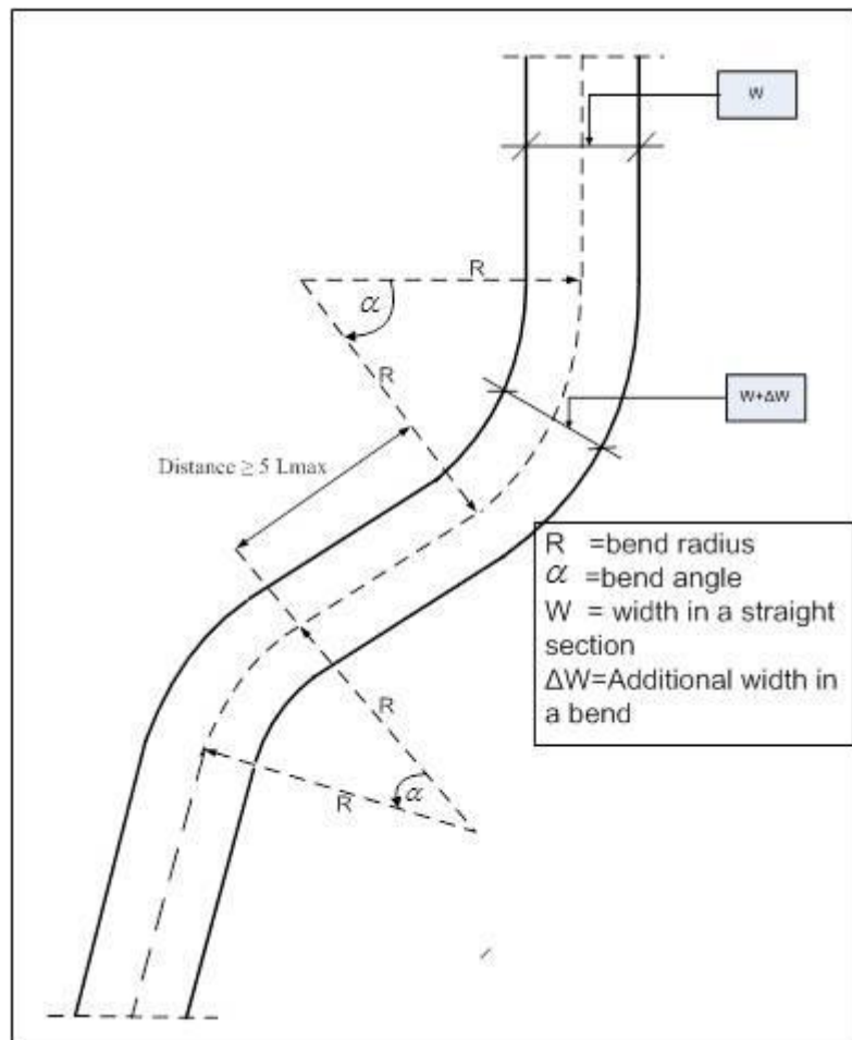
Figure 3.3: Bend configuration
